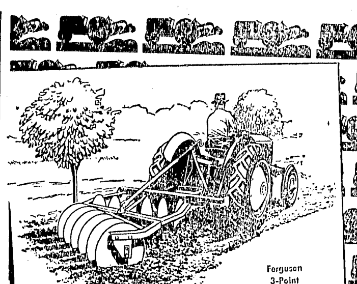
Ferguson 3-Point Attachment
